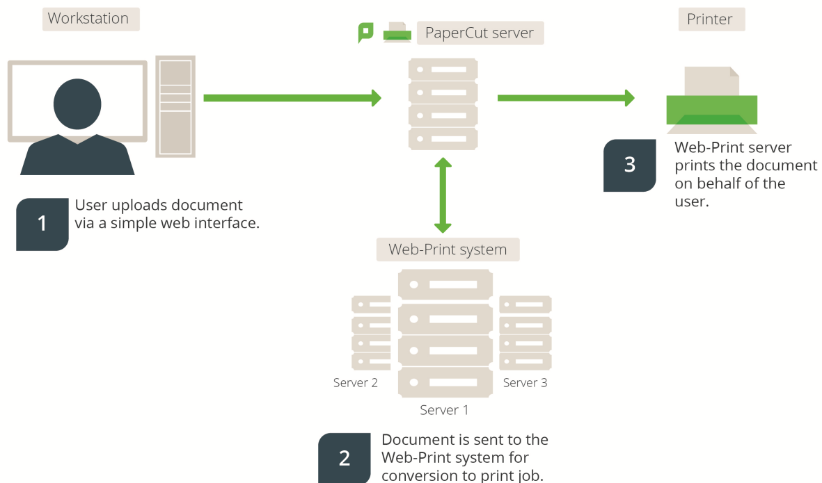
Figure 52: Web Print architecture overview
